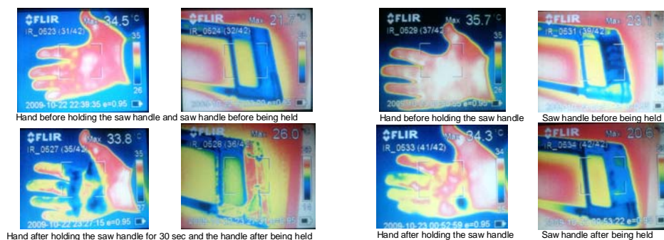
Figure 2: The cold surface of a metallic saw handle absorbs the skin heat (see the 4 thermo-images on the left). If the handle is insulated with a special tape, the heat remains on the hand.
